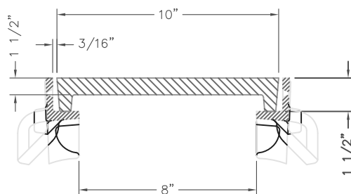
R-4999-BX TYPICAL SECTION TYPE "D" LID w/ TYPE "B" FRAME (SCALE: 1/4"=1")
